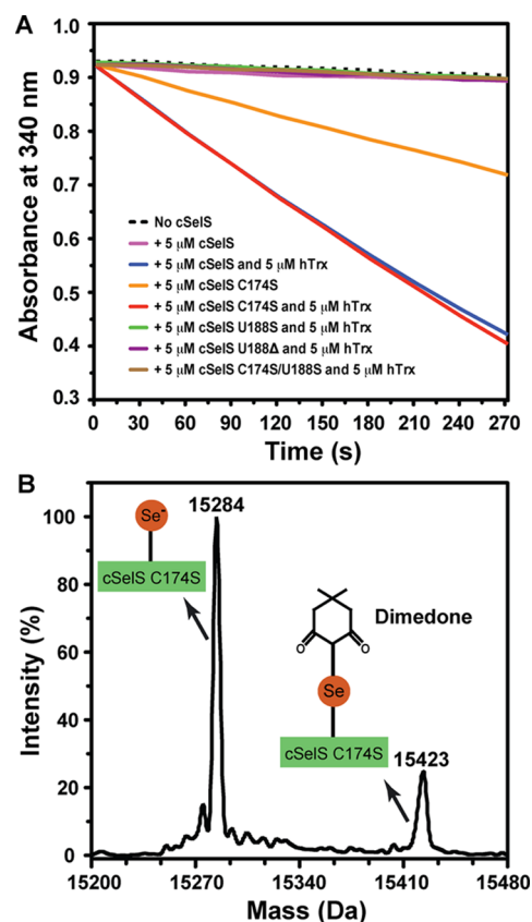
Figure 1. (A) Identification of the peroxidatic and resolving residues in SelS using peroxidase assays. NADPH consumption is monitored in the presence of 8 nM hTrxR, 5 μM hTrx, and 200 μM \text{H}_2\text{O}_2 , and 5 μM of either wild-type cSelS, C174S, U188S, or U188Δ mutants. (B) Trapping of the reaction intermediate, selenenic acid, in cSelS C174S. Mass spectrum showing cSelS C174S (15284 Da) and its dimedone adduct (15423 Da).
