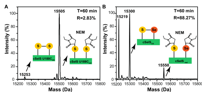
Figure 2. Electrospray ionization mass spectrometry-based detection of the rate of formation of the selenenylsulfide bond in cSelS and the disulfide bond in cSelS U188C. (A) After 60 min, the majority of cSelS U188C was still reduced, allowing for full alkylation by NEM. Molecular masses are 15253 Da for oxidized cSelS U188C and 15505 Da for alkylated cSelS U188C. (B) After 60 min, the majority of cSelS was oxidized. Molecular masses are 15219 Da for alkylated cSelS U188Δ (a truncated, inactive form that arises during expression), 15300 Da for oxidized cSelS, and 15550 Da for alkylated cSelS. R denotes the percent of oxidized protein.
