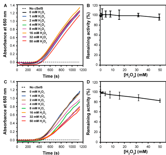
Figure 3. Resistance of cSelS to inactivation by \text{H}_2\text{O}_2 . The ability of cSelS to reduce insulin's intermolecular disulfide bond following incubations with \text{H}_2\text{O}_2 is monitored by recording the increasing turbidity caused by insulin's chain B aggregation. (A) cSelS reductase activity assay after incubations with \text{H}_2\text{O}_2 . (B) Percentage of the remaining activity of wild-type cSelS after treatment with \text{H}_2\text{O}_2 . (C) cSelS C174S reductase activity assay after incubations with \text{H}_2\text{O}_2 . (D) Percentage of the remaining activity of cSelS C174S after treatment with \text{H}_2\text{O}_2 . The error bars represent the range of measurements (that is, highest and lowest values) among two repetitions, using two independent protein preparations.
